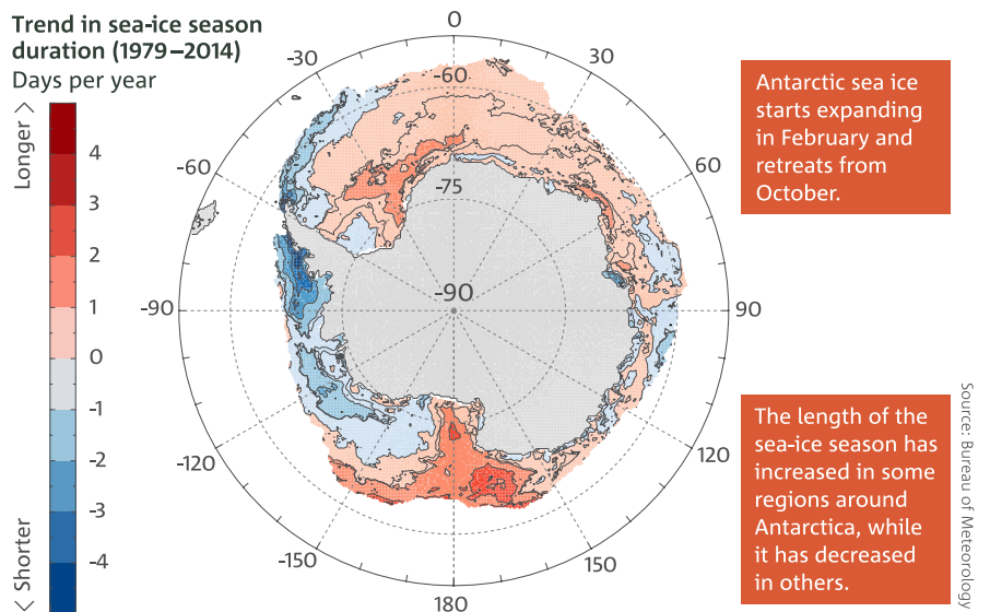
Trends in the length of the sea-ice season duration each year (in days per year) around Antarctica, 1979–2014. The Antarctic land-mass is shaded grey. Each year sea-ice around Antarctica expands (or advances) from a minimum extent in February to a maximum extent in September. Duration is a measure of the number of days that a particular location contains sea-ice.
