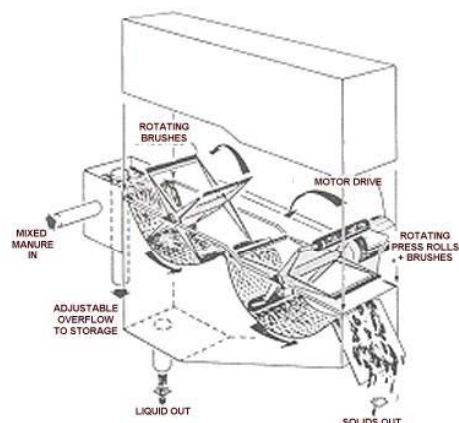
Diagram displaying the function of a Brush Screen with Press-Rolls
