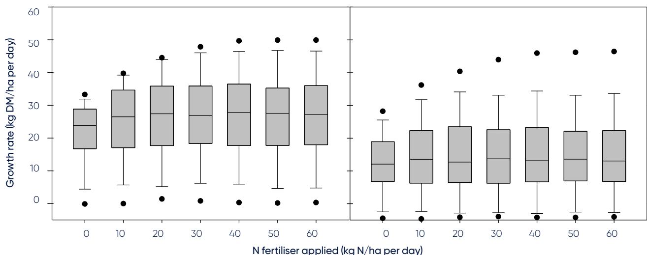
Figure 1 Autumn pasture growth rate responses to N fertiliser at Ellinbank, West Gippsland (left), and Terang, SW Victoria (right), in autumn (March, April, May) between 2000 and 2017. The middle line shows the median response, boxes show the response for the years between the 25th and 75th percentile of years, whiskers show the responses for the 10th and 90th percentile of years and dots show the extremes.
