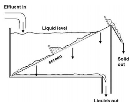
Diagram of a Flighted Conveyor Screen
